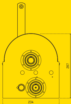
15:1 CAR TRAILER BRAKE WINCH DIMENSIONS
